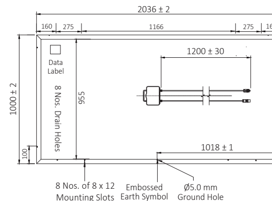
Module Dimension Diagram (mm) SGalactic
